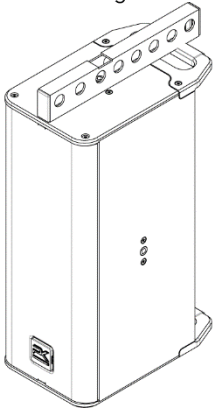
Vertical Hang
