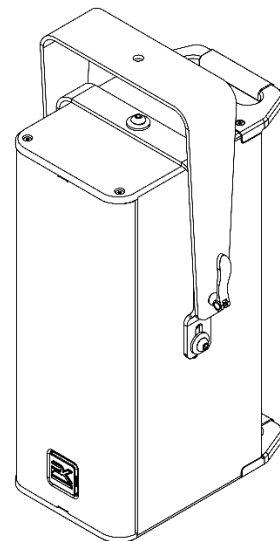
SUSPENDED MOUNT
