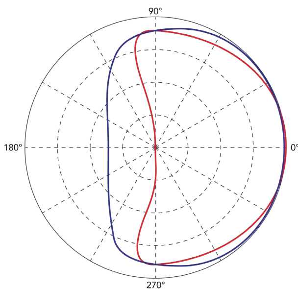
T218 Cardioid Dispersion Pattern (FBF)
