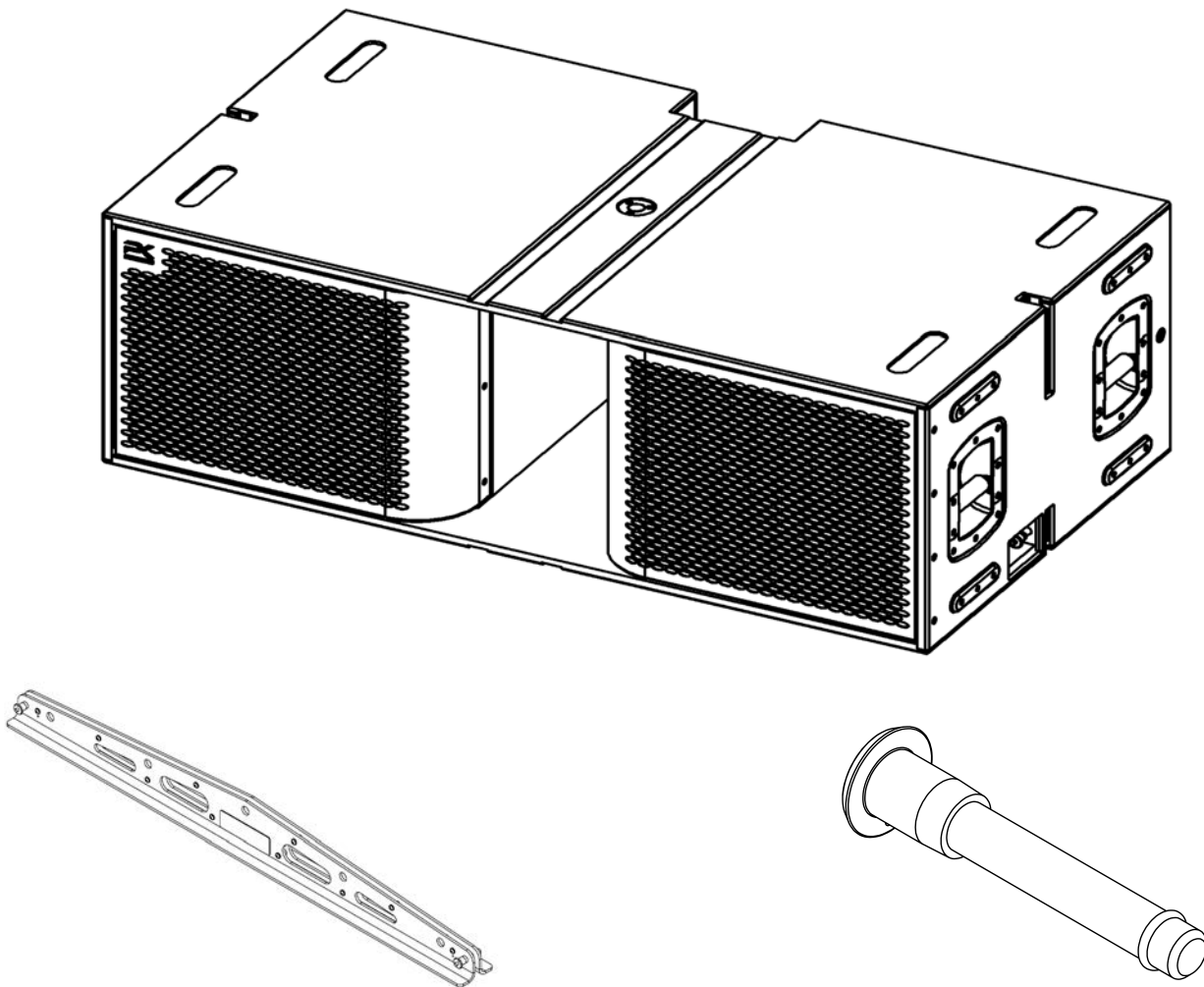
T218 Suspension Frame
