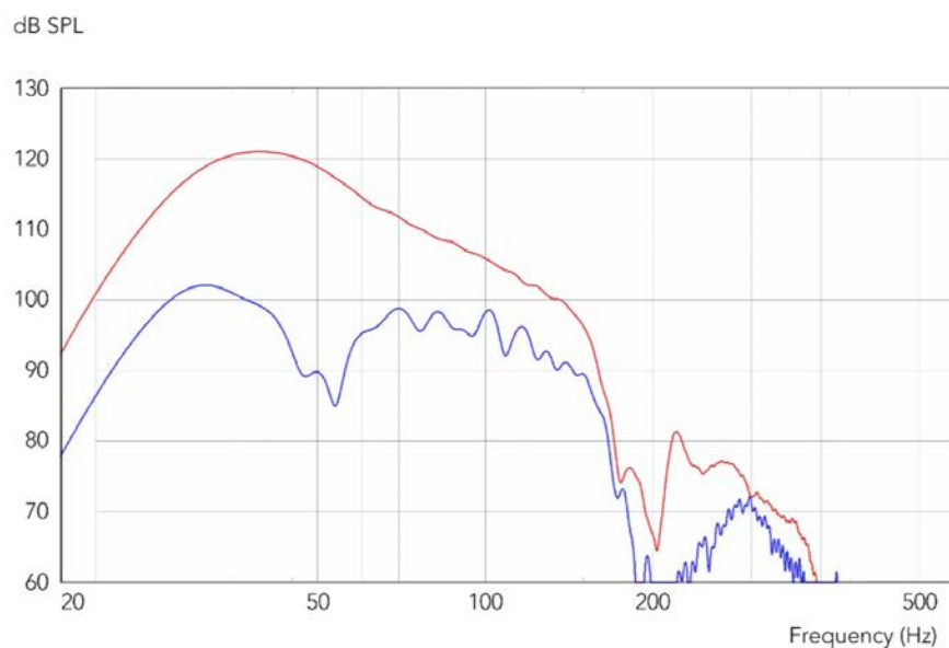
T218 Frequency Response - Regular & Cardioid
